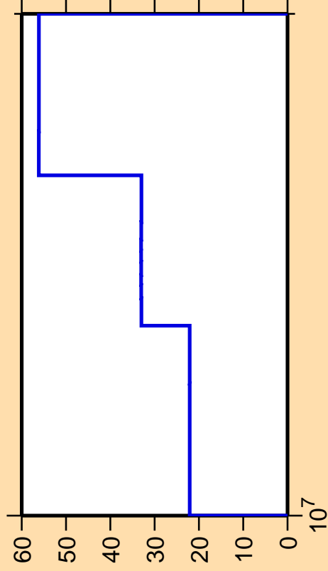
\Delta\sigma/\sigma vs. E for ^{162}\text{Hf}(n,ncont.)
