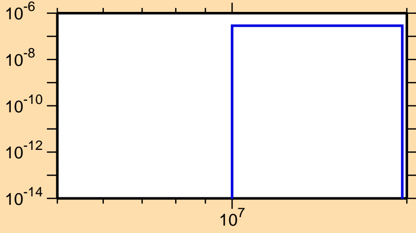
\sigma vs. E for ^{162}\text{Hf}(\text{mt } 45)
