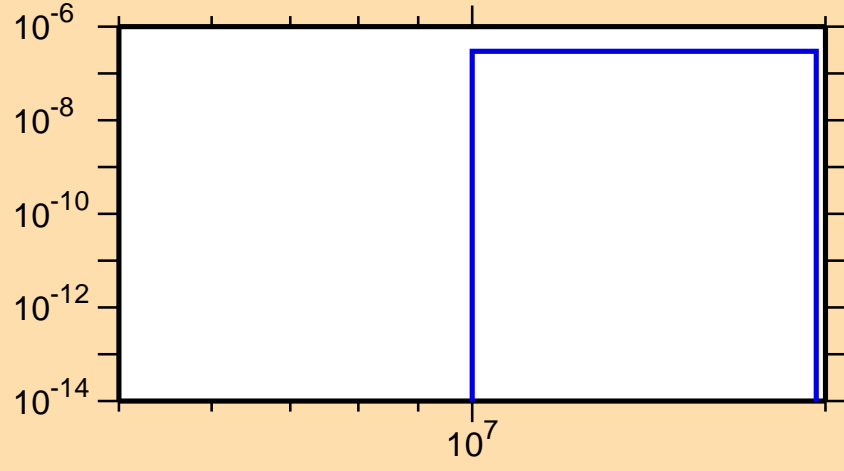
\sigma vs. E for ^{162}\text{Hf}(n,\text{pd})
