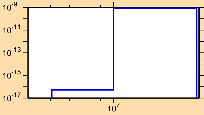
\sigma vs. E for ^{162}\text{Hf}(\text{mt117})
