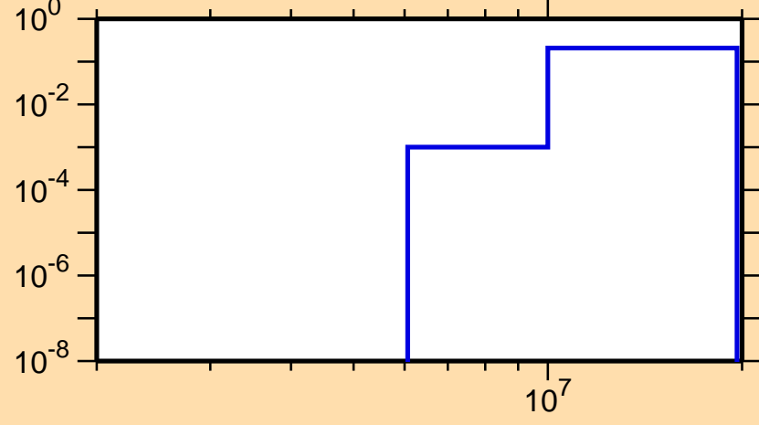
\sigma vs. E for ^{162}\text{Hf}(n,np)
