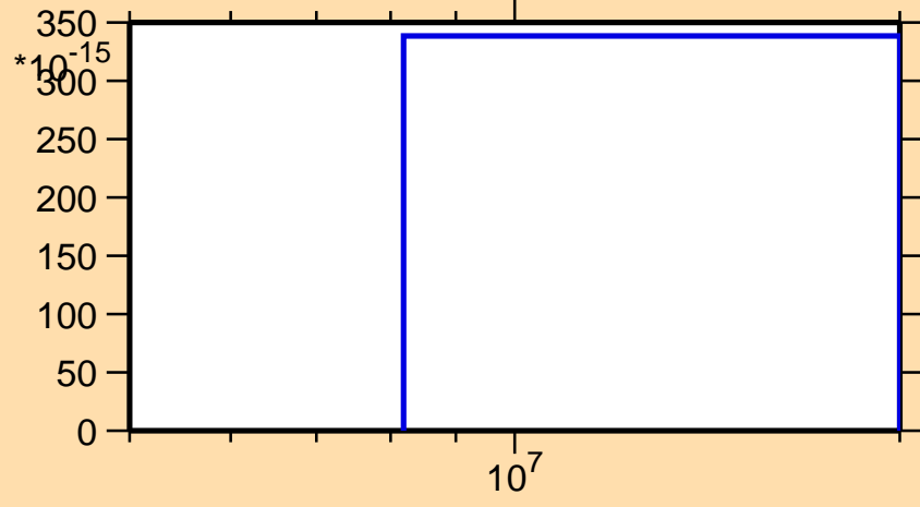
\sigma vs. E for ^{162}\text{Hf}(\text{mt } 34)
