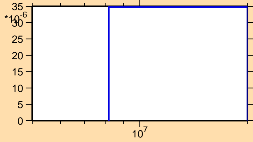
\sigma vs. E for ^{162}\text{Hf}(n,t)
