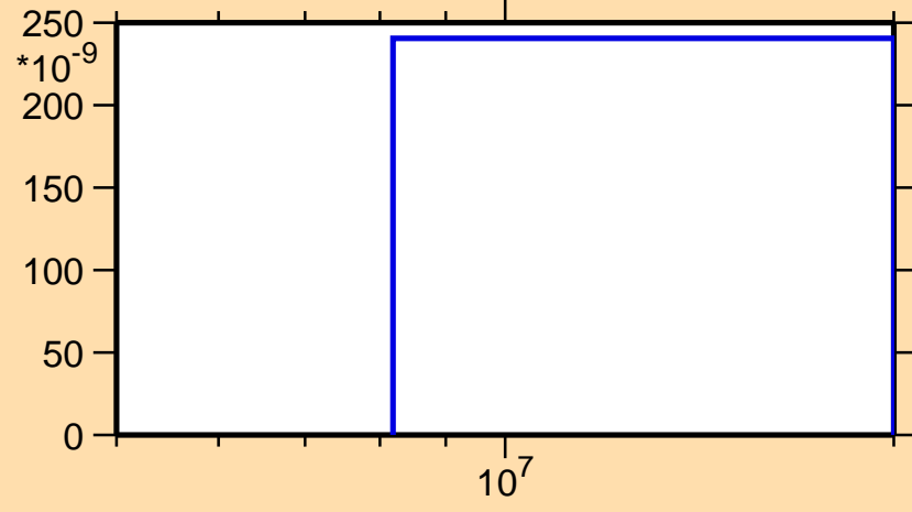
\sigma vs. E for ^{162}\text{Hf}(n,\text{pd})
