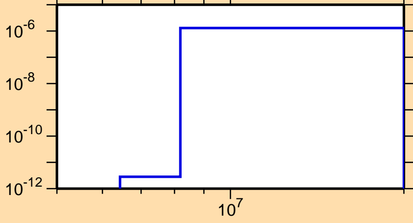
\sigma vs. E for ^{162}\text{Hf}(n,\text{He}3)
