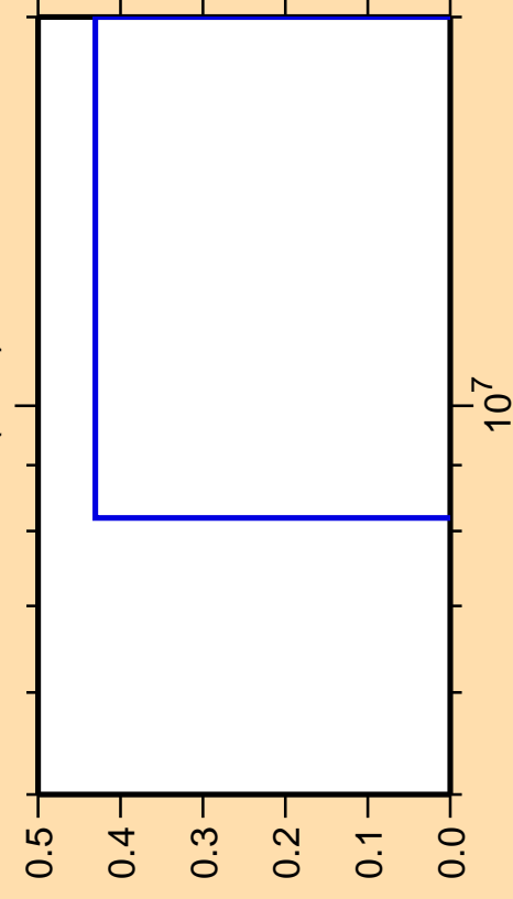
\Delta\sigma/\sigma vs. E for ^{162}\text{Hf}(n,nt)
