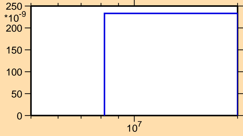
\sigma vs. E for ^{162}\text{Hf}(\text{mt } 45)
