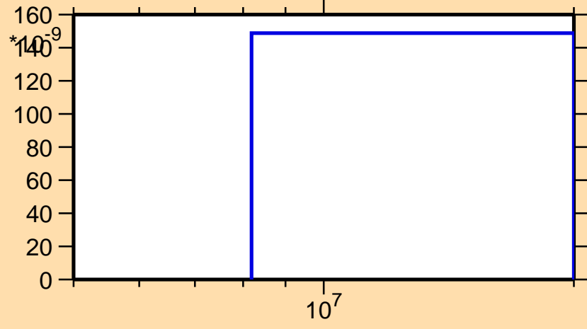
\sigma vs. E for ^{162}\text{Hf}(n,2n\alpha)
