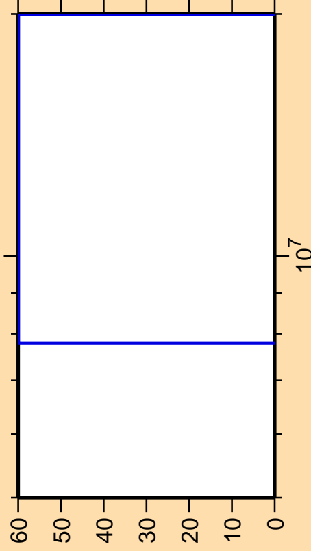
\Delta\sigma/\sigma vs. E for ^{163}\text{Hf}(n,2n)
