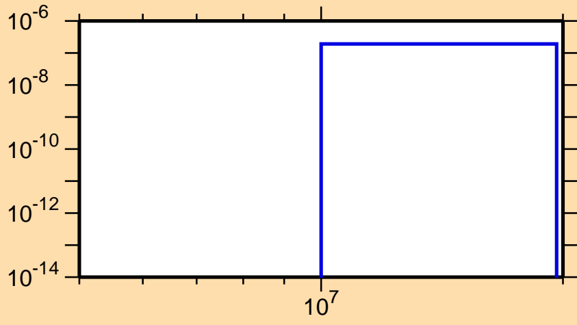
\sigma vs. E for ^{163}\text{Hf}(\text{mt } 45)
