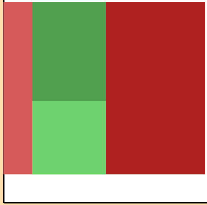
\Delta\sigma/\sigma vs. E for ^{163}\text{Hf}(n,\text{inel.})
