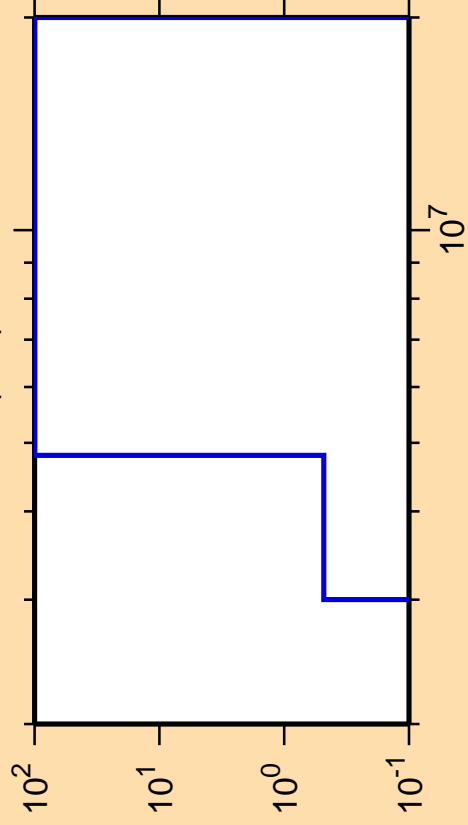
\Delta\sigma/\sigma vs. E for ^{163}\text{Hf}(n,d)
