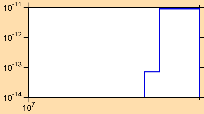
\sigma vs. E for ^{164}\text{Hf} (mt 34)
