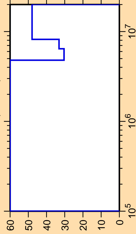
\Delta\sigma/\sigma vs. E for ^{164}\text{Hf}(n,\text{inel.})
