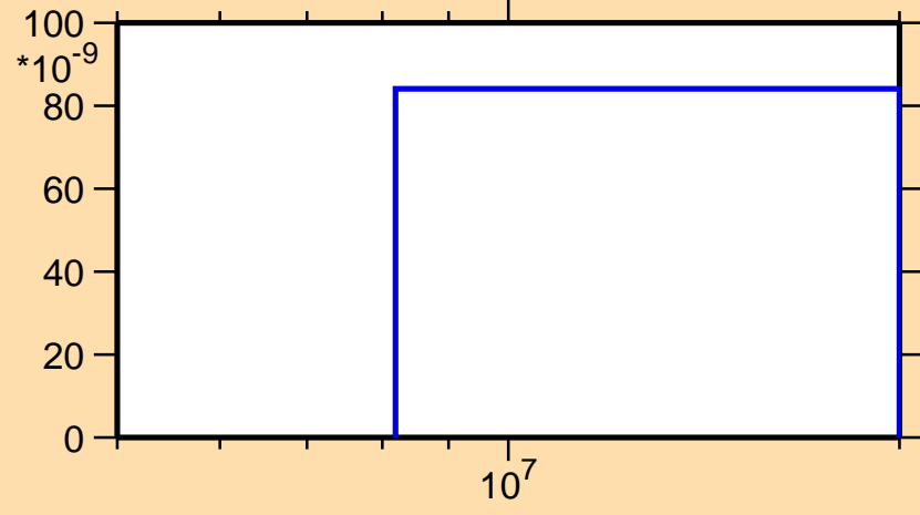
\sigma vs. E for ^{164}\text{Hf}(n,2n\alpha)
