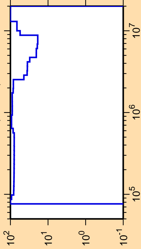
\Delta\sigma/\sigma vs. E for ^{165}\text{Hf}(n,\text{inel.})
