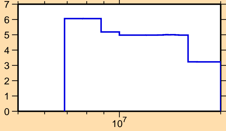
\Delta\sigma/\sigma vs. E for ^{167}\text{Hf}(n,\text{nonel.})
