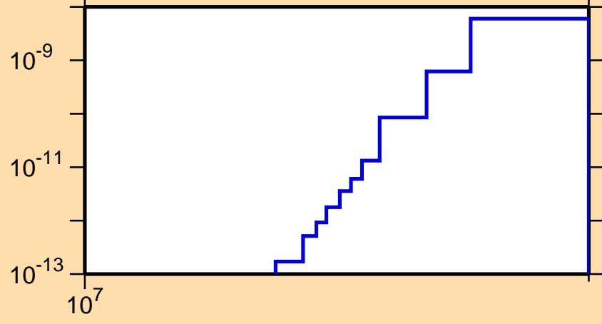
\sigma vs. E for ^{167}\text{Hf(mt 45)}
