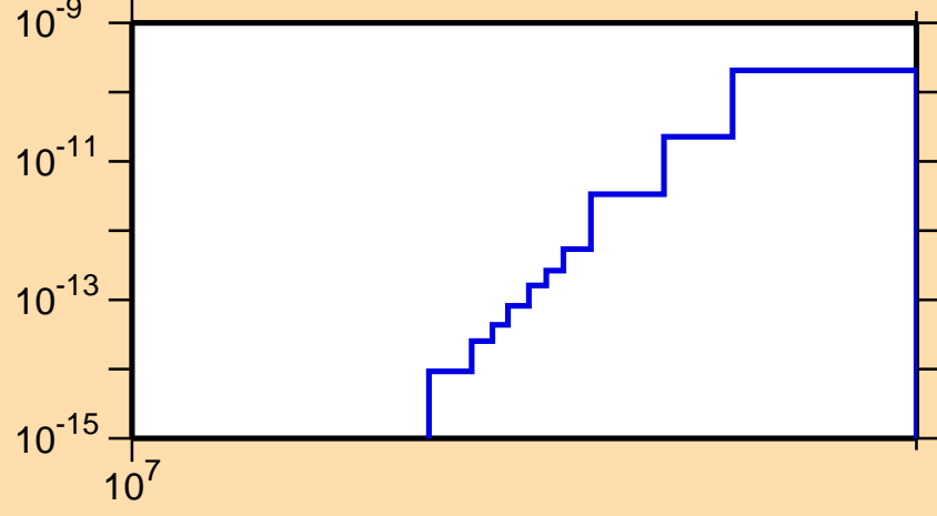
\sigma vs. E for ^{167}\text{Hf(mt117)}
