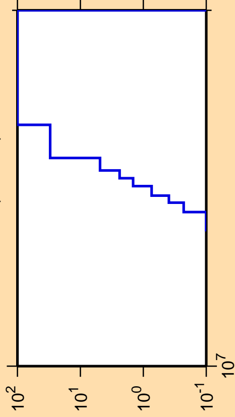
\Delta\sigma/\sigma vs. E for ^{167}\text{Hf(mt117)}
