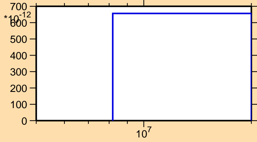
\sigma vs. E for ^{167}\text{Hf}(n,pd)
