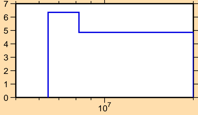
\Delta\sigma/\sigma vs. E for ^{167}\text{Hf}(n,\text{el.})
