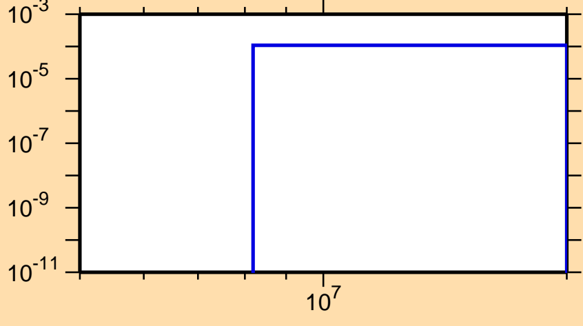
\sigma vs. E for ^{167}\text{Hf}(n,t)
