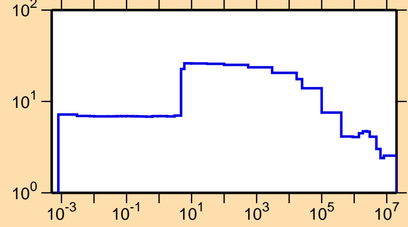
\sigma vs. E for ^{167}\text{Hf}(n,\text{el.})
