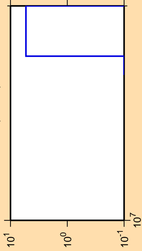
\Delta\sigma/\sigma vs. E for ^{168}\text{Hf} (mt 34)
