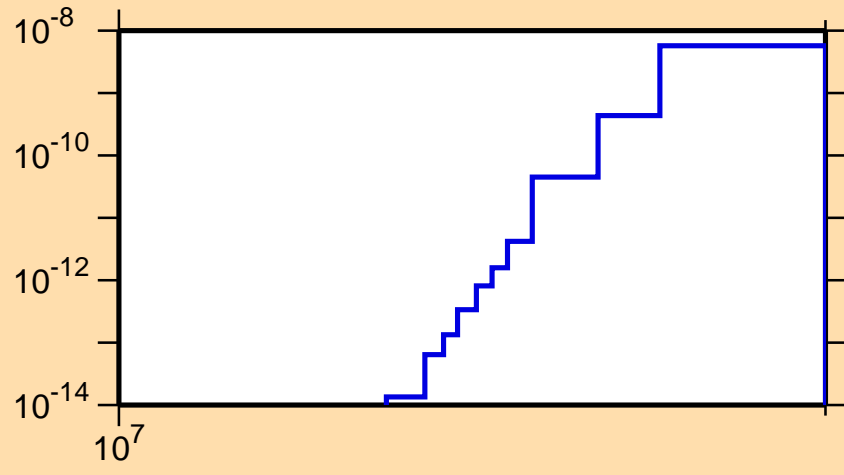
\sigma vs. E for ^{168}\text{Hf}(n,pd)
