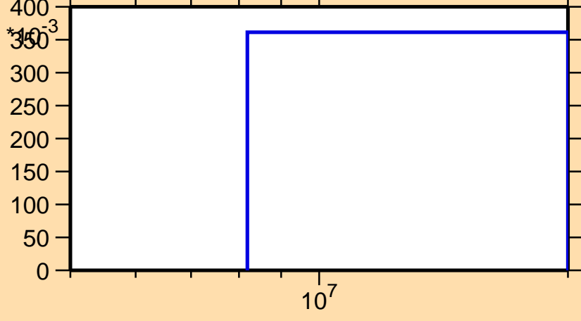
\sigma vs. E for ^{168}\text{Hf}(n,2n)
