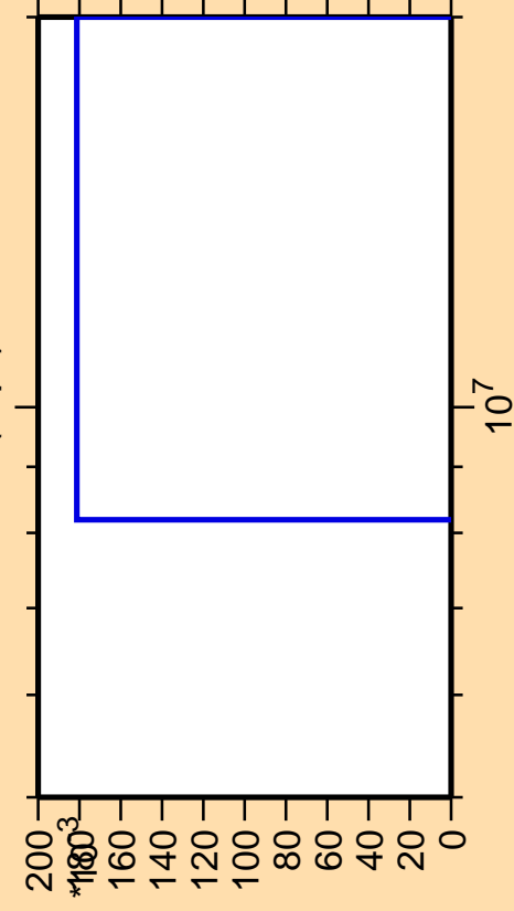
\Delta\sigma/\sigma vs. E for ^{168}\text{Hf}(n,\text{pt})
