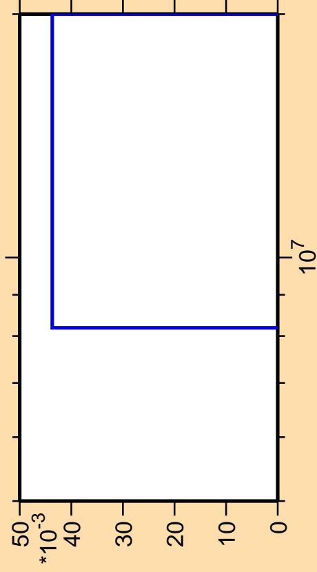
\Delta\sigma/\sigma vs. E for ^{168}\text{Hf}(\text{mt } 34)
