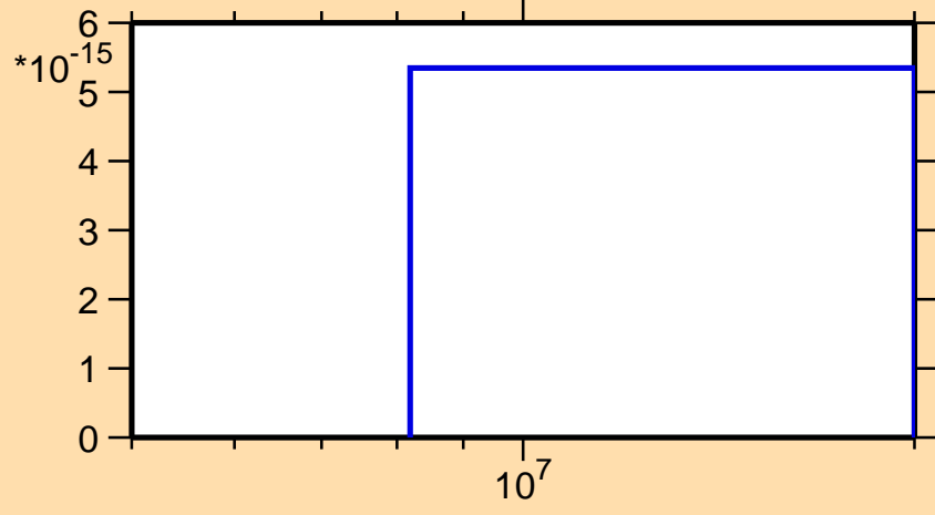
\sigma vs. E for ^{168}\text{Hf}(\text{mt } 34)
