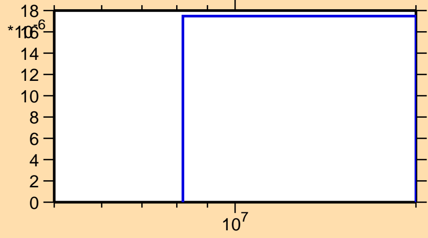
\sigma vs. E for ^{168}\text{Hf}(n,t)
