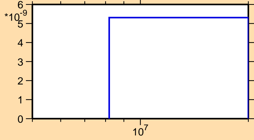
\sigma vs. E for ^{168}\text{Hf}(n,2np)
