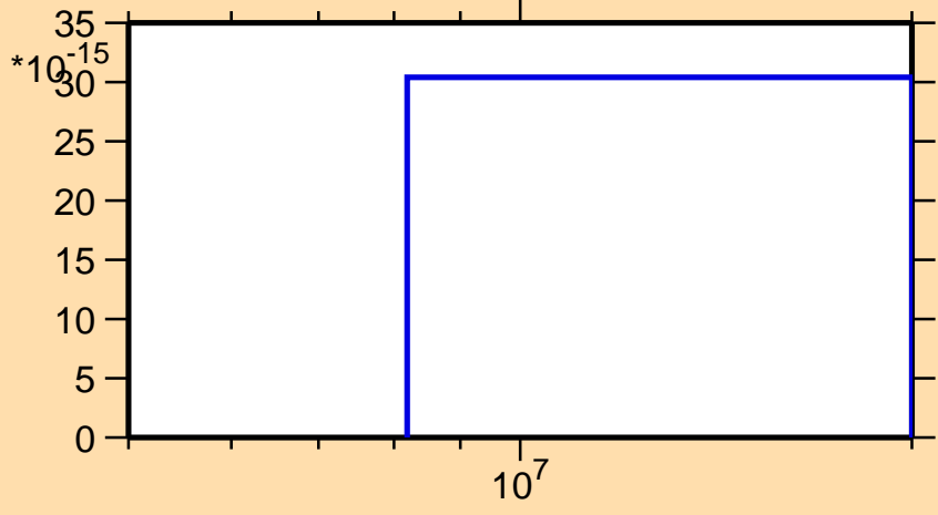
\sigma vs. E for ^{168}\text{Hf}(n,\text{pt})
