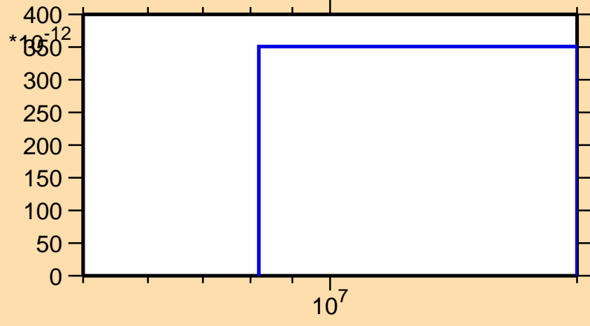
\sigma vs. E for ^{168}\text{Hf}(n,nd)
