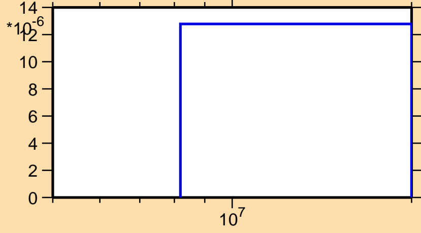
\sigma vs. E for ^{168}\text{Hf}(n,3n)
