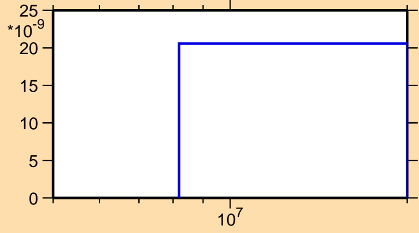
\sigma vs. E for ^{168}\text{Hf}(n,\text{He3})
