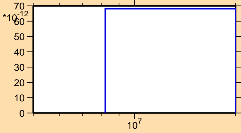
\sigma vs. E for ^{168}\text{Hf}(\text{mt } 45)
