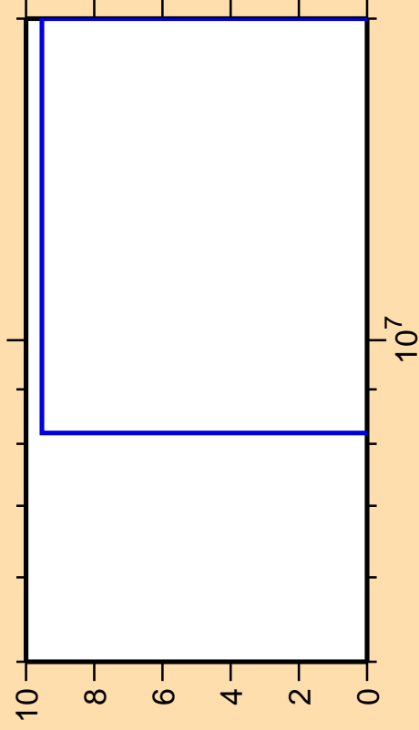
\Delta\sigma/\sigma vs. E for ^{169}\text{Hf}(\text{mt } 34)
