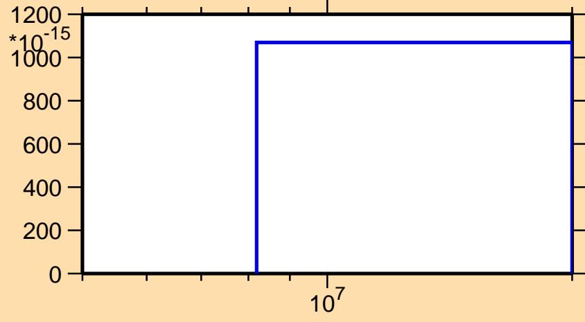
\sigma vs. E for ^{169}\text{Hf}(\text{mt } 34)
