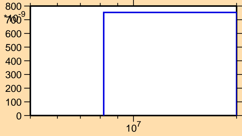
\sigma vs. E for ^{169}\text{Hf}(n,2np)
