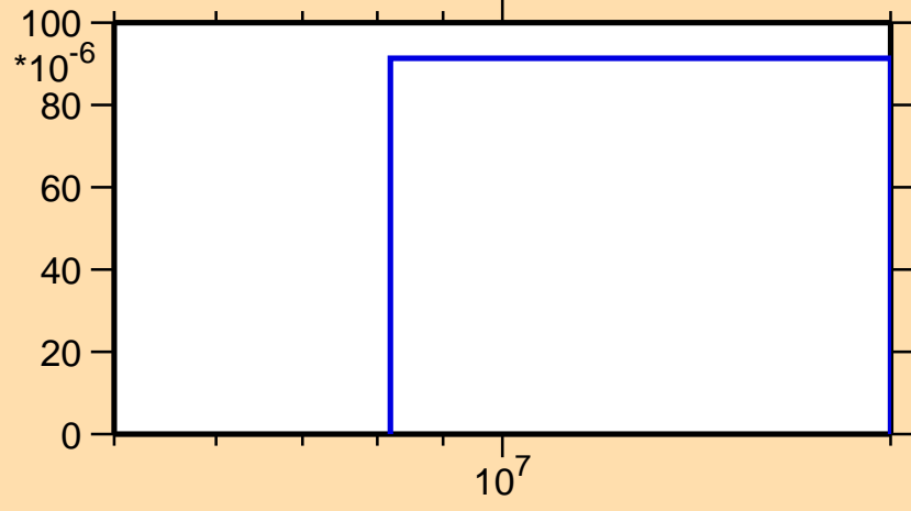
\sigma vs. E for ^{169}\text{Hf}(n,t)
