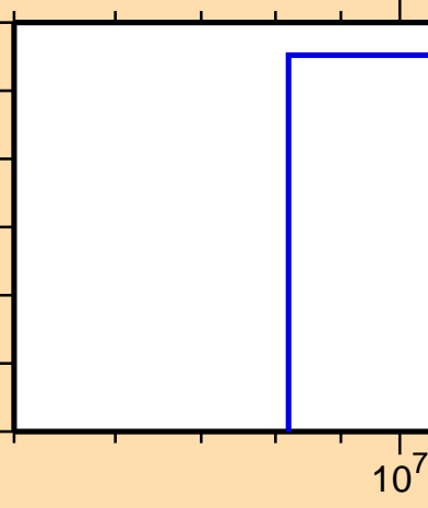
\sigma vs. E for ^{169}\text{Hf}(\text{mt117})
