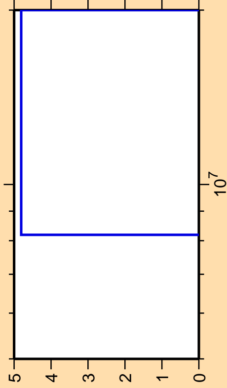
\Delta\sigma/\sigma vs. E for ^{169}\text{Hf} (mt 45)
