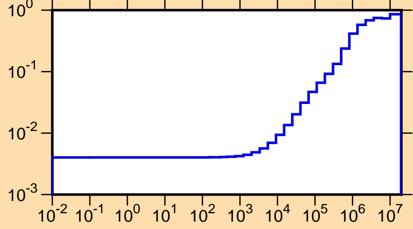
\mu vs. E for ^{170}\text{Hf}(\text{mt251})
