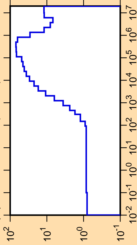
\Delta\mu/\mu vs. E for ^{170}\text{Hf}(\text{mt251})
