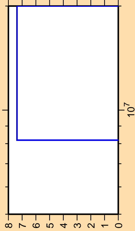
\Delta\sigma/\sigma vs. E for ^{170}\text{Hf}(n,\text{pd})
