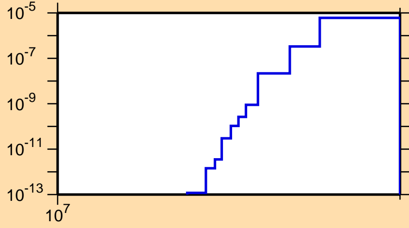
\sigma vs. E for ^{171}\text{Hf}(n,\text{nd})
