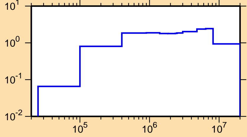
\sigma vs. E for ^{171}\text{Hf}(n,\text{inel.})
