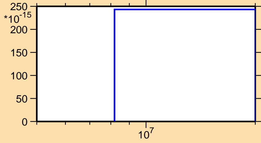
\sigma vs. E for ^{171}\text{Hf}(\text{mt } 45)
