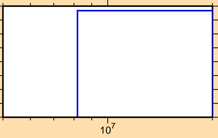
\sigma vs. E for ^{171}\text{Hf}(n,t)
