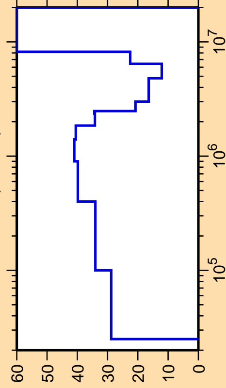
\Delta\sigma/\sigma vs. E for ^{171}\text{Hf}(n,\text{inel.})
