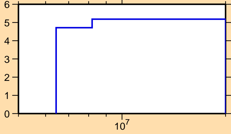
\Delta\sigma/\sigma vs. E for ^{171}\text{Hf}(n,\text{tot.})
