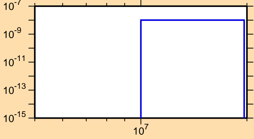
\sigma vs. E for ^{171}\text{Hf}(n,\text{He}3)
