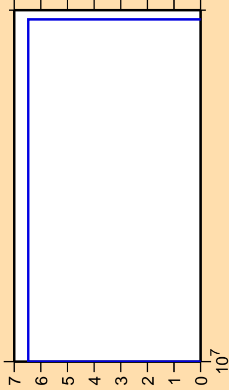
\Delta\sigma/\sigma vs. E for ^{171}\text{Hf}(n,\text{pt})
