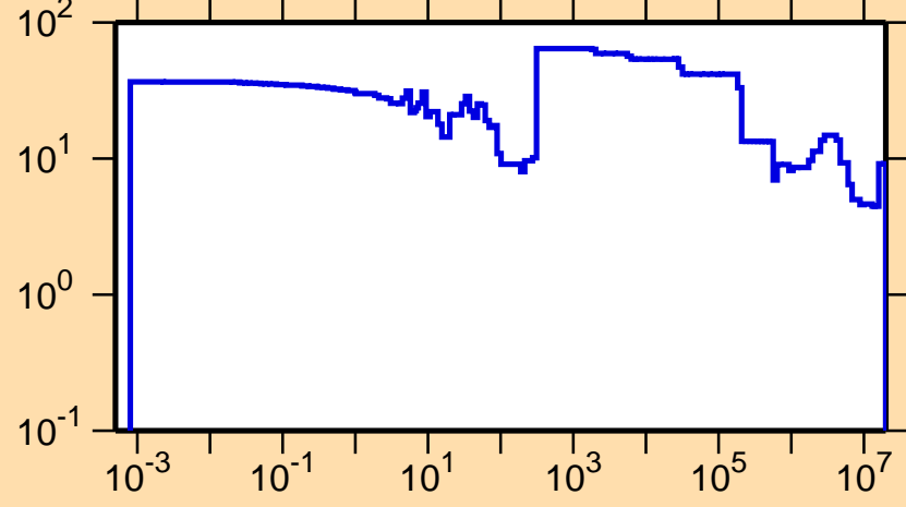
\Delta\sigma/\sigma vs. E for ^{172}\text{Hf}(n,\text{tot.})
