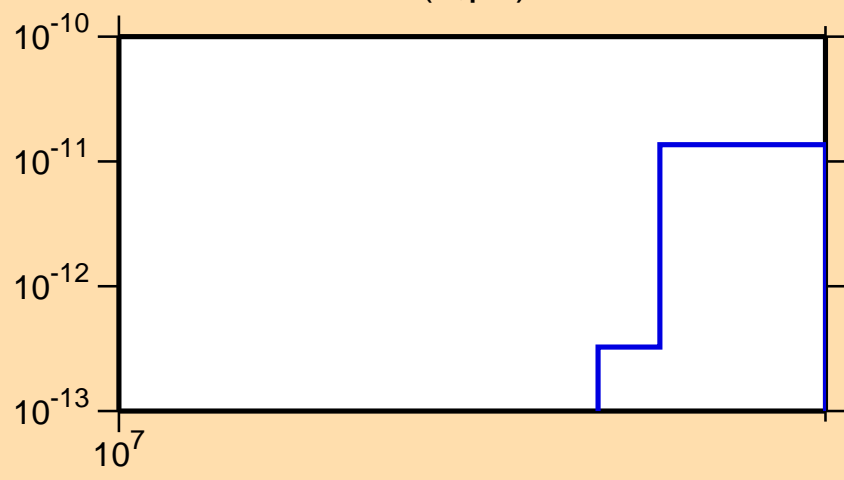
\sigma vs. E for ^{172}\text{Hf}(n,pd)
