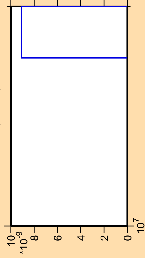
\Delta\sigma/\sigma vs. E for ^{172}\text{Hf}(\text{mt } 11)
