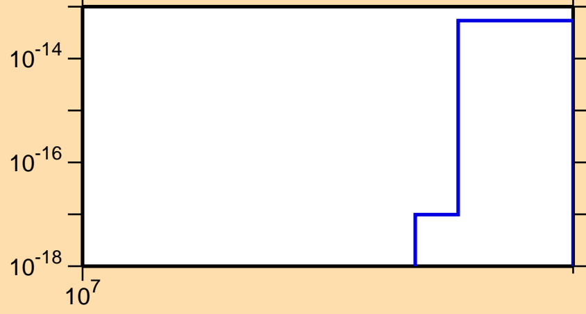
\sigma vs. E for ^{172}\text{Hf} (mt 34)
