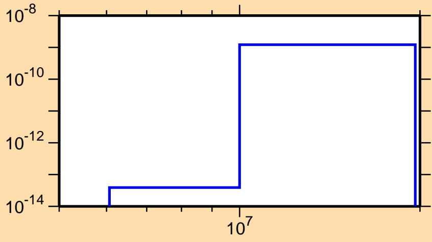
\sigma vs. E for ^{172}\text{Hf}(n,p\alpha)
