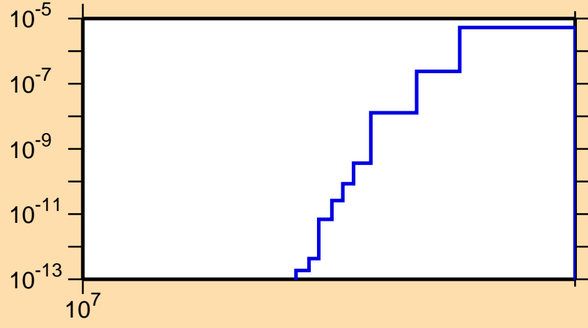
\sigma vs. E for ^{173}\text{Hf}(n,nd)
