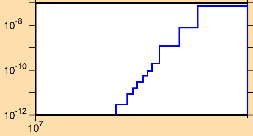
\sigma vs. E for ^{173}\text{Hf}(n,\text{He3})
