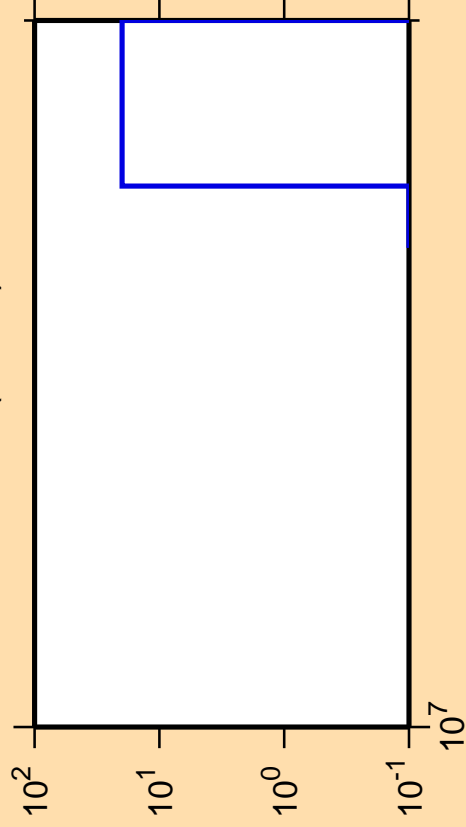
\Delta\sigma/\sigma vs. E for ^{173}\text{Hf} (mt 34)
