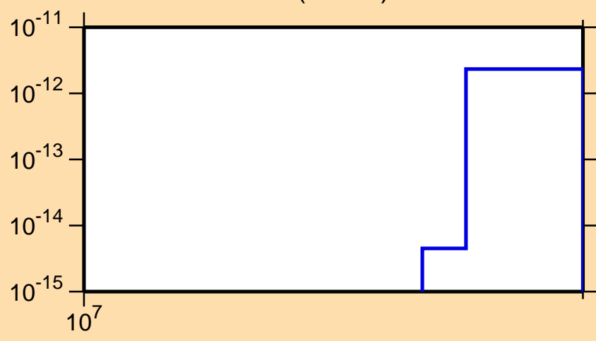
\sigma vs. E for ^{173}\text{Hf} (mt 34)
