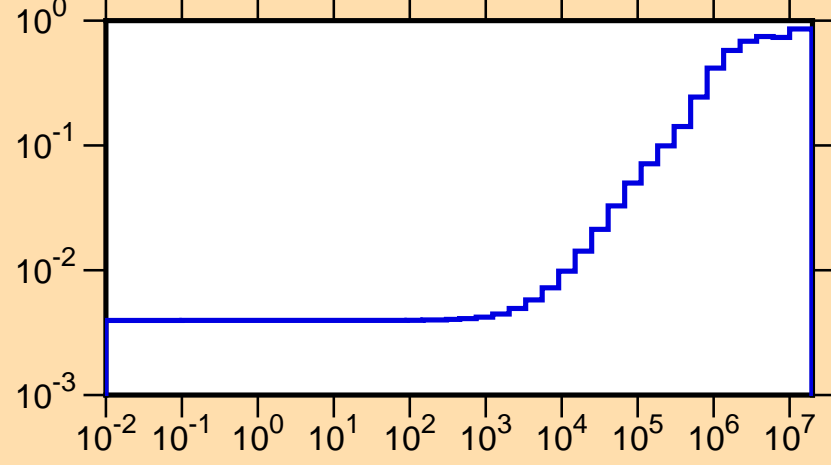
\mu vs. E for ^{173}\text{Hf}(\text{mt251})
