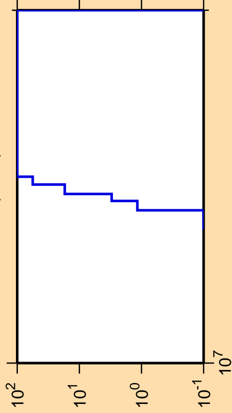
\Delta\sigma/\sigma vs. E for ^{175}\text{Hf}(n,nd)
