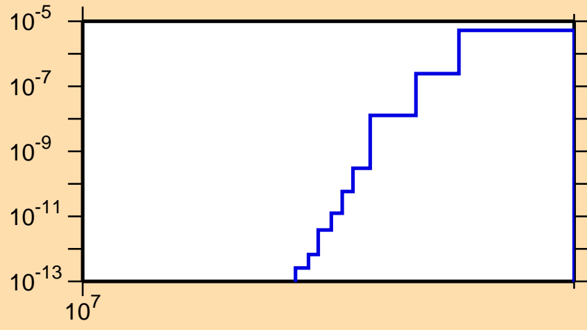
\sigma vs. E for ^{175}\text{Hf}(n,nd)
