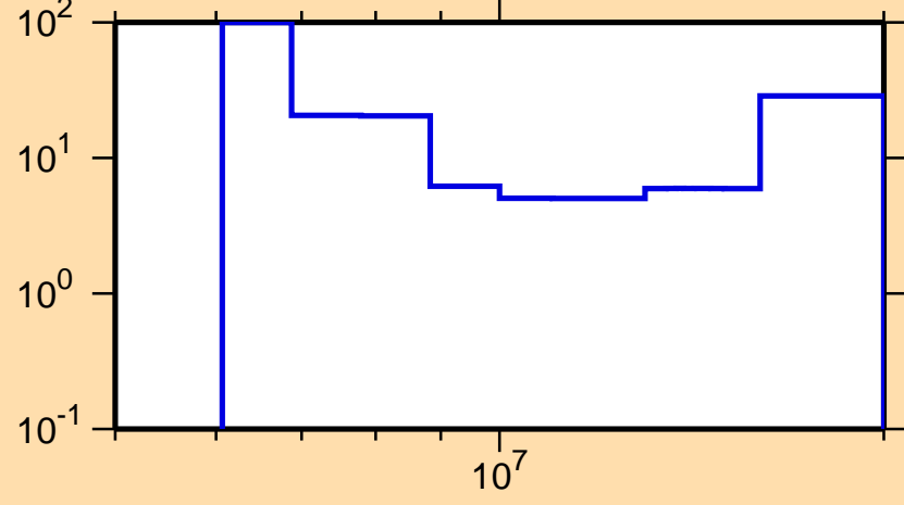
\Delta\sigma/\sigma vs. E for ^{175}\text{Hf}(n,2n)
