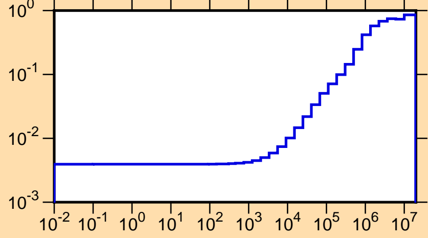
\mu vs. E for ^{175}\text{Hf}(\text{mt251})
