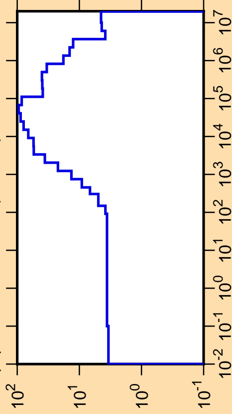
\Delta\mu/\mu vs. E for ^{175}\text{Hf}(\text{mt251})
