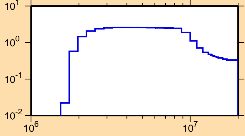
\sigma vs. E for ^{176}\text{Hf}(n,n\text{cont.})
