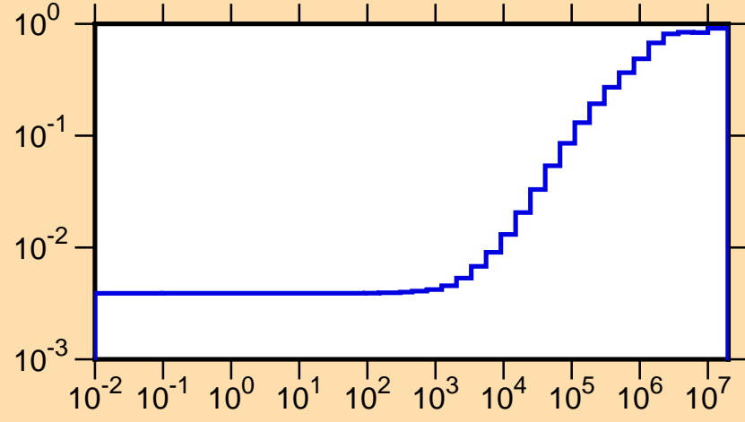
\mu vs. E for ^{176}\text{Hf}(\text{mt251})
