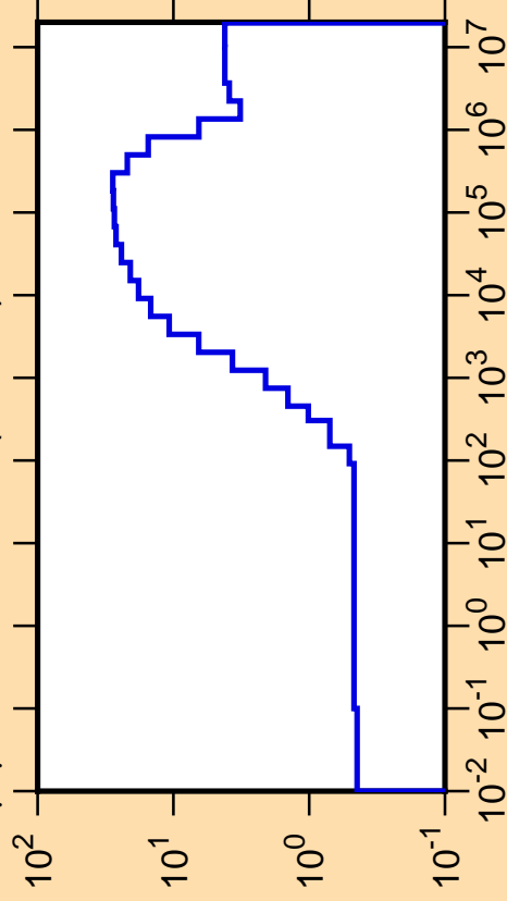
\Delta\mu/\mu vs. E for ^{176}\text{Hf}(\text{mt251})
