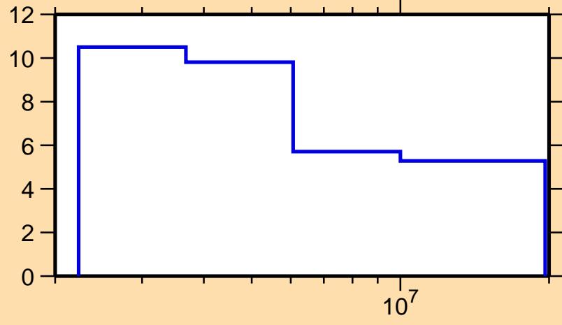
\Delta\sigma/\sigma vs. E for ^{176}\text{Hf}(n,el.)
