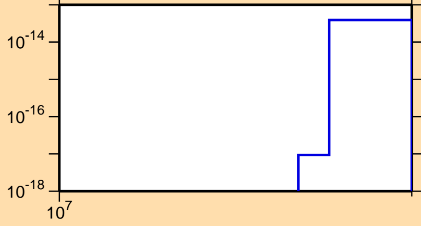
\sigma vs. E for ^{177}\text{Hf} (mt 34)
