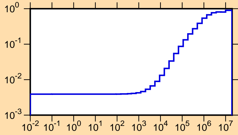
\mu vs. E for ^{177}\text{Hf}(\text{mt251})
