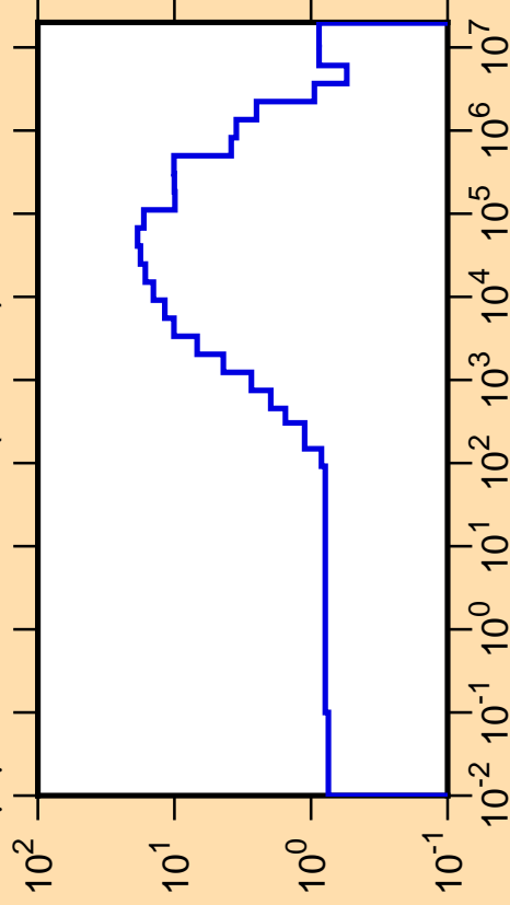
\Delta\mu/\mu vs. E for ^{177}\text{Hf}(\text{mt251})
