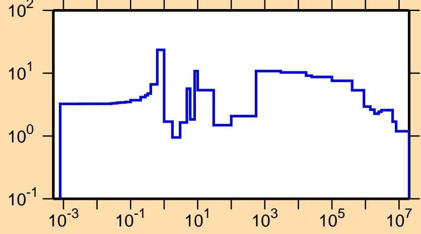
\Delta\sigma/\sigma vs. E for ^{177}\text{Hf}(n,\text{tot.})
