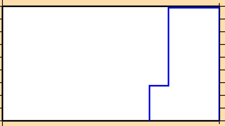
\sigma vs. E for ^{177}\text{Hf}(n,p\alpha)
