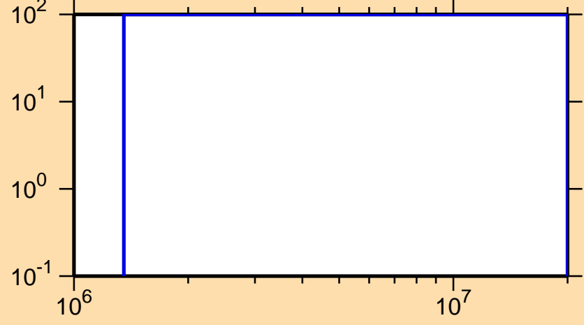
\Delta\sigma/\sigma vs. E for ^{177}\text{Hf}(n, n_1)
