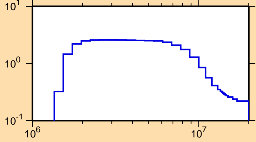
\sigma vs. E for ^{177}\text{Hf}(n,n\text{cont.})
