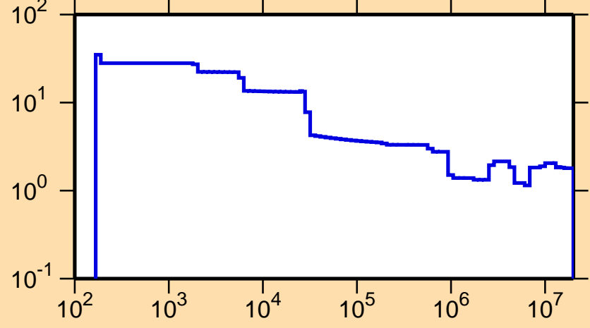
\Delta\sigma/\sigma vs. E for ^{177}\text{Hf}(n,\text{el.})
