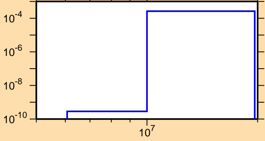
\sigma vs. E for ^{177}\text{Hf}(n,t)
