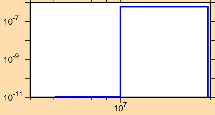
\sigma vs. E for ^{177}\text{Hf}(n,2n\alpha)
