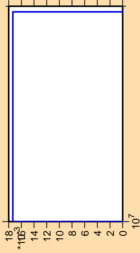
\Delta\sigma/\sigma vs. E for ^{177}\text{Hf} (mt 45)
