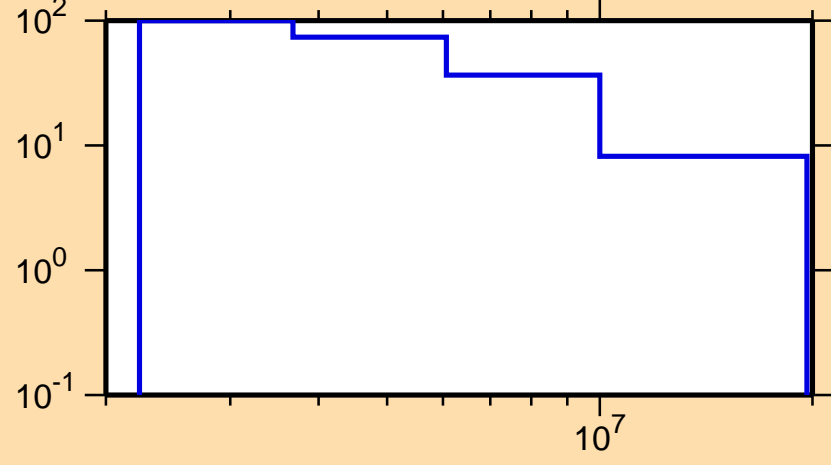
\Delta\sigma/\sigma vs. E for ^{177}\text{Hf}(n,2n)
