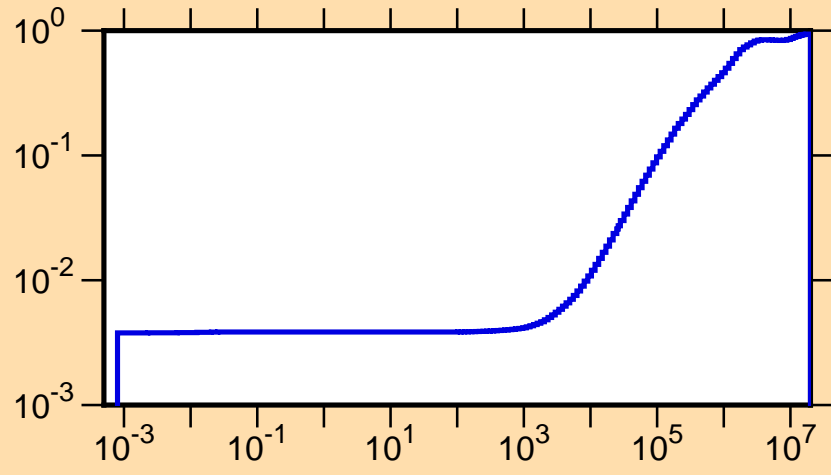
\mu vs. E for ^{178}\text{Hf}(\text{mt251})
