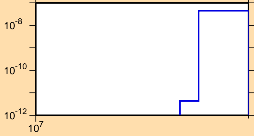
\sigma vs. E for ^{178}\text{Hf}(n,2np)
