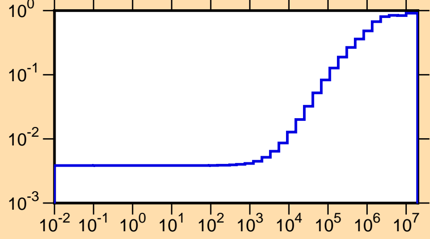
\mu vs. E for ^{178}\text{Hf}(\text{mt251})
