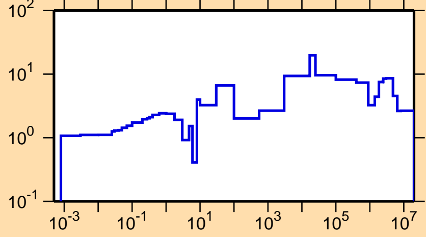
\Delta\sigma/\sigma vs. E for ^{178}\text{Hf}(n,\text{tot.})
