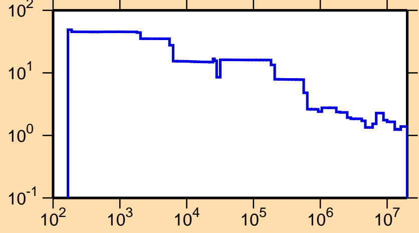
\Delta\sigma/\sigma vs. E for ^{178}\text{Hf}(n,\text{nonel.})
