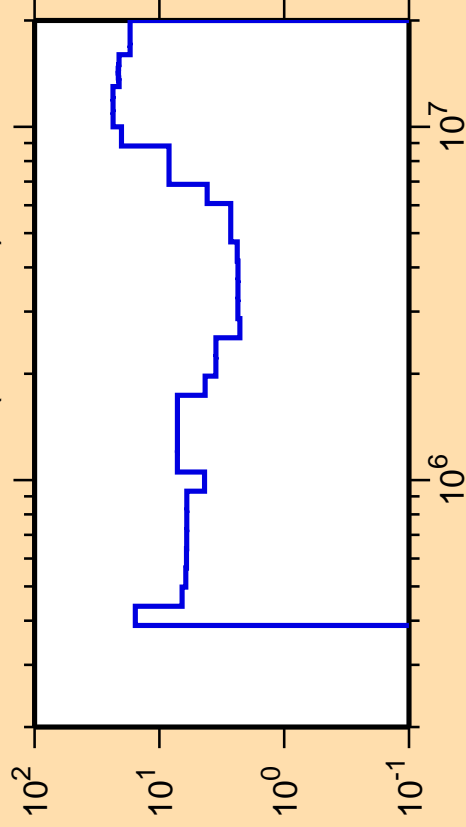
\Delta\sigma/\sigma vs. E for ^{178}\text{Hf}(n, ncont.)
