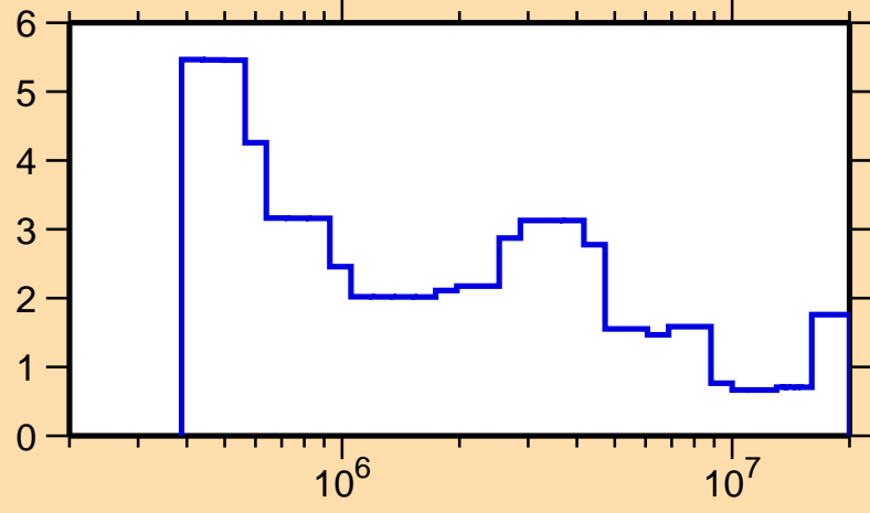
\Delta\sigma/\sigma vs. E for ^{178}\text{Hf}(n, tot.)
