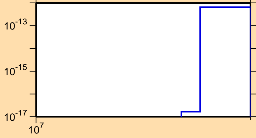
\sigma vs. E for ^{178}\text{Hf}(n,3n\alpha)
