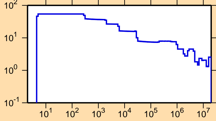
\Delta\sigma/\sigma vs. E for ^{178}\text{Hf}(n,\text{el.})
