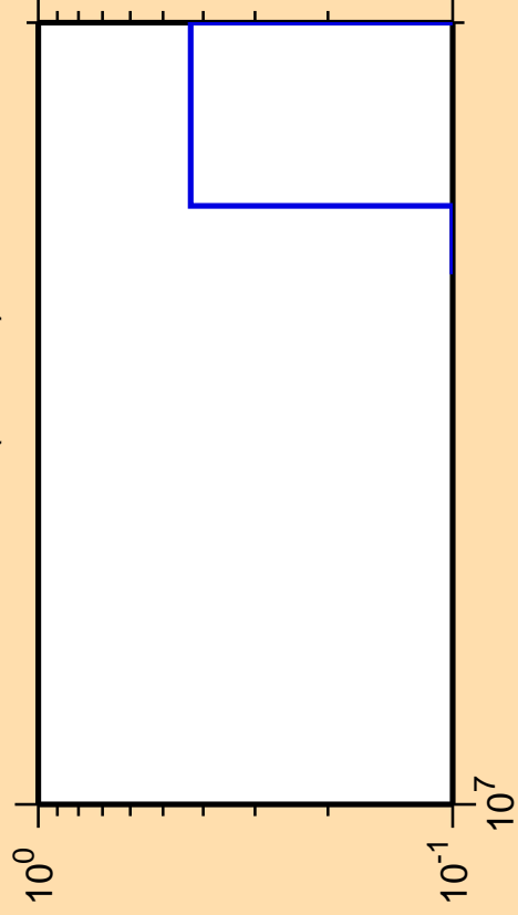
\Delta\sigma/\sigma vs. E for ^{178}\text{Hf} (mt 34)
