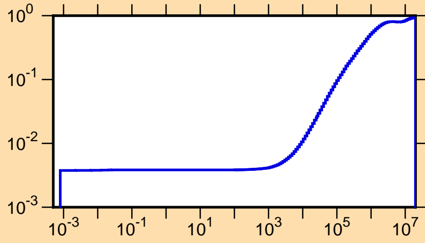
\mu vs. E for ^{179}\text{Hf}(\text{mt251})
