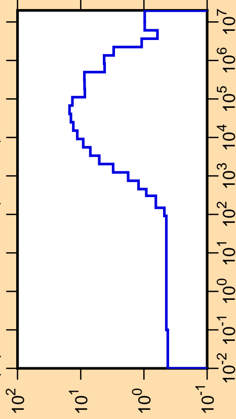
\Delta\mu/\mu vs. E for ^{179}\text{Hf}(\text{mt251})
