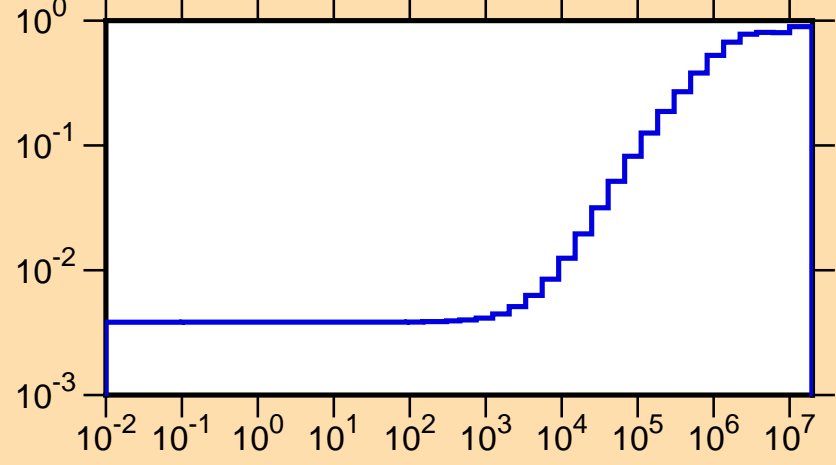
\mu vs. E for ^{179}\text{Hf}(\text{mt251})
