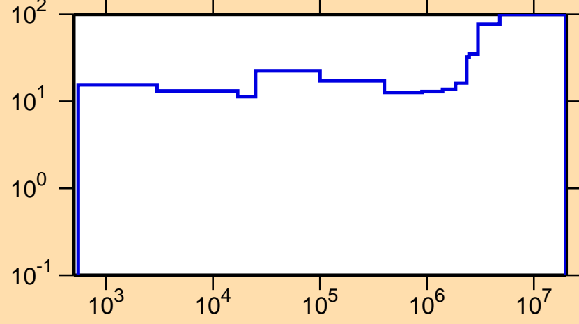
\Delta\sigma/\sigma vs. E for ^{179}\text{Hf}(n,n_1)
