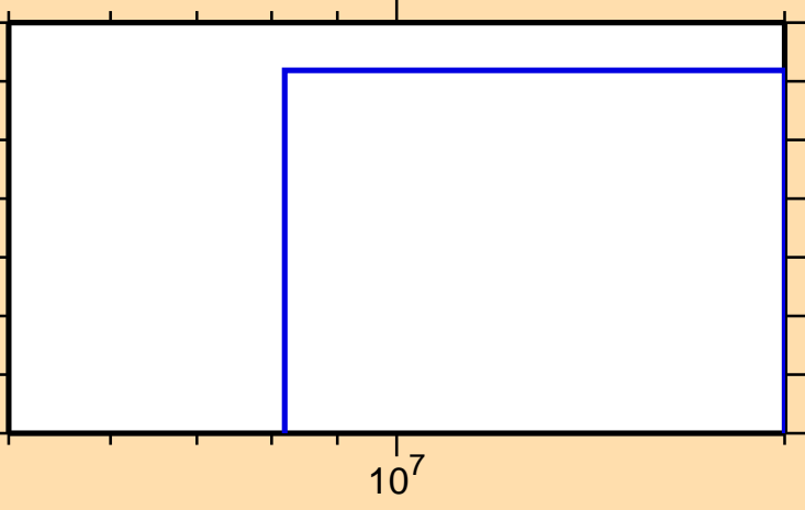
\sigma vs. E for ^{179}\text{Hf}(\text{mt } 11)
