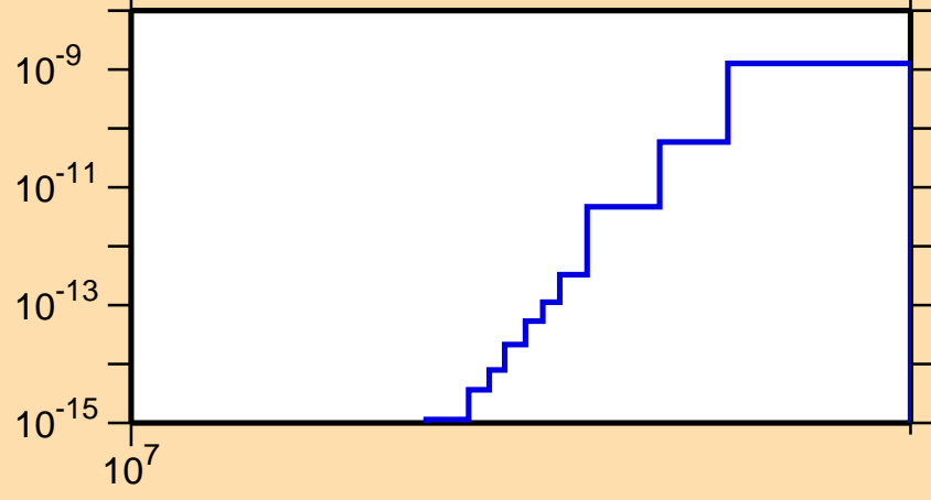
\sigma vs. E for ^{179}\text{Hf}(n,\text{He3})
