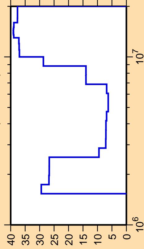
\Delta\sigma/\sigma vs. E for ^{180}\text{Hf}(n,\text{ncont.})
