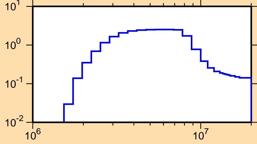
\sigma vs. E for ^{180}\text{Hf}(n,n\text{cont.})
