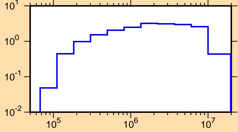
\sigma vs. E for ^{180}\text{Hf}(n,\text{inel.})
