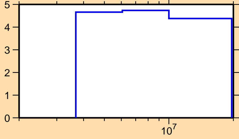
\Delta\sigma/\sigma vs. E for ^{180}\text{Hf}(n,\text{nonel.})
