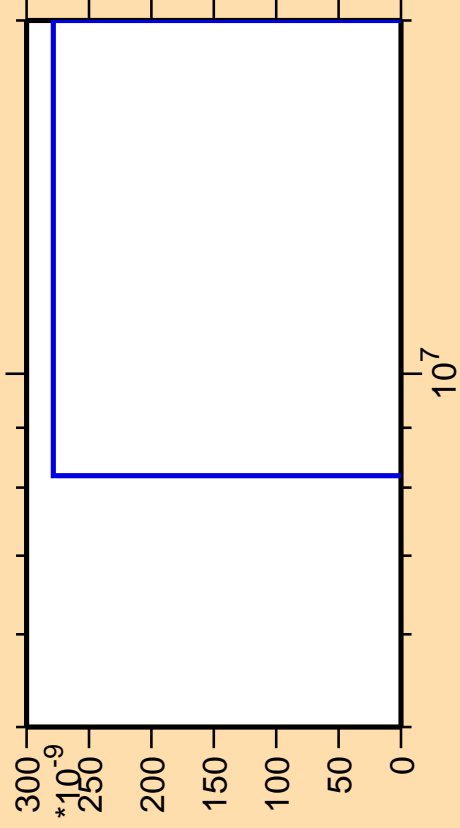
\Delta\sigma/\sigma vs. E for ^{180}\text{Hf}(\text{mt } 11)
