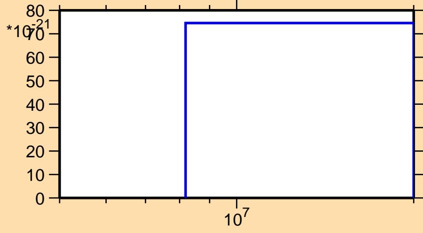
\sigma vs. E for ^{180}\text{Hf}(\text{mt } 11)
