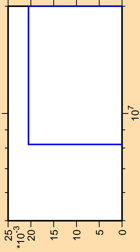
\Delta\sigma/\sigma vs. E for ^{180}\text{Hf}(n,3n\alpha)
