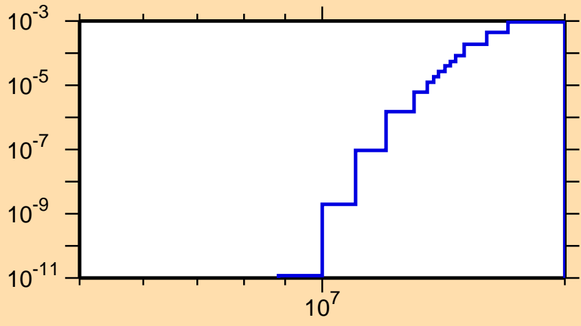
\sigma vs. E for ^{180}\text{Hf}(n,t)
