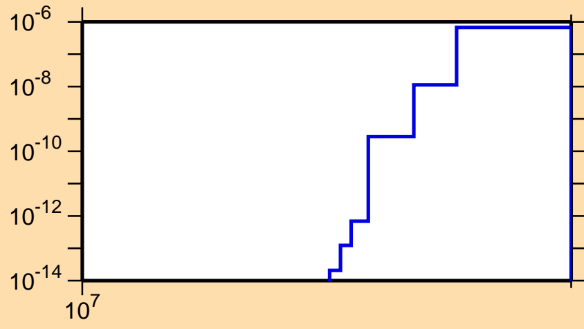
\sigma vs. E for ^{180}\text{Hf}(n,nd)
