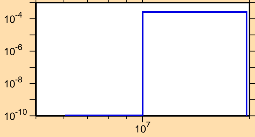
\sigma vs. E for ^{180}\text{Hf}(n,d)
