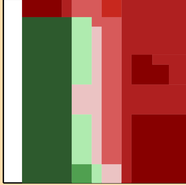
\Delta\sigma/\sigma vs. E for ^{181}\text{Hf}(n,p)
